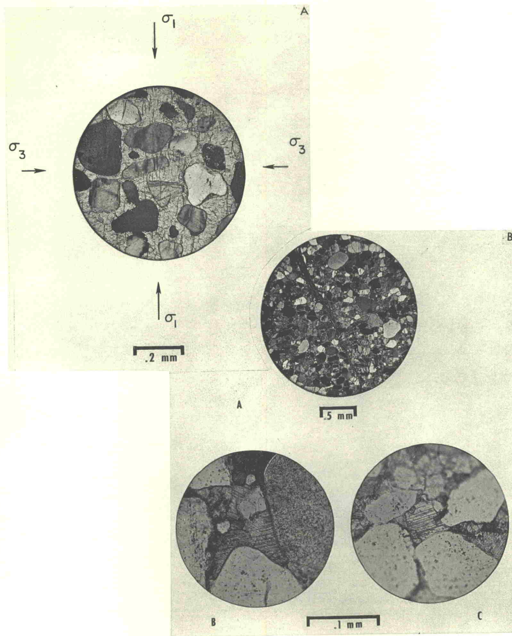
Thin section cut of specimen 725
